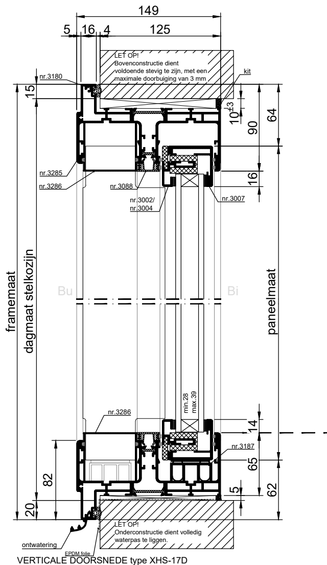
VERTICALE DOORSNEDE type XHS-17D
