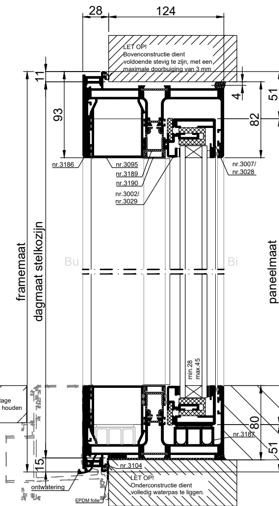
VERTICALE DOORSNEDE type XHS-10D
