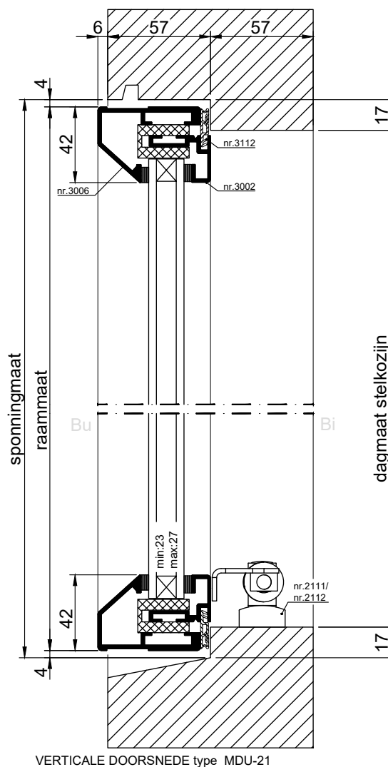
VERTICALE DOORSNEDE type MDU-21
